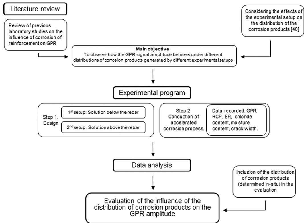
Fig. 1. Research methodology.
