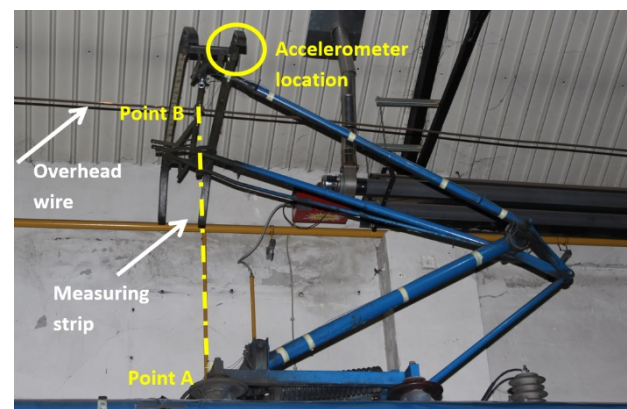
Fig. 4. Overhead wire height and shock measurement setup.
