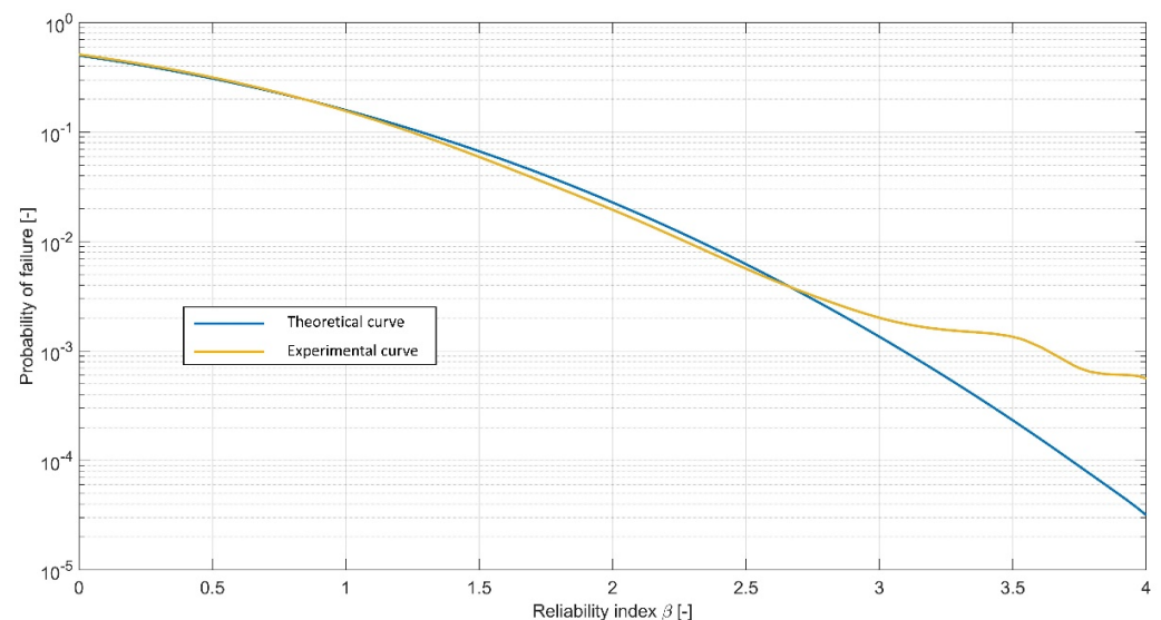
Figure 10. Probabilities of failure and respective reliability indices for levee slope stability.
