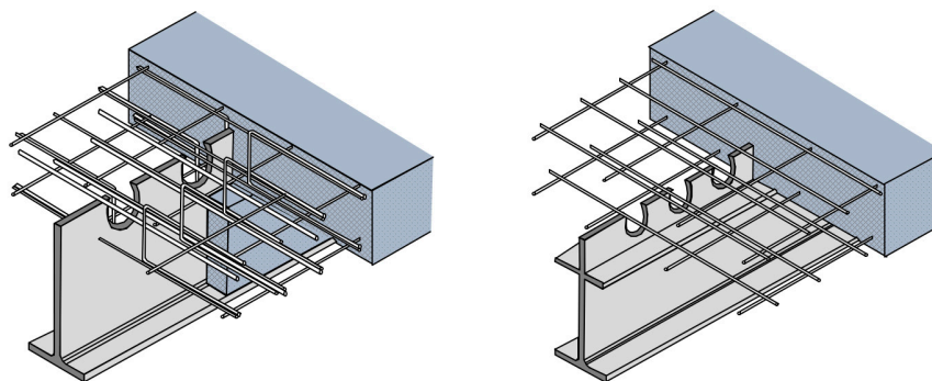
Figure 2. Possible solutions with composite dowel rib connectors.
