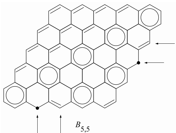
Figure 18. More second most important structures in the same rhombic nanoflake.
