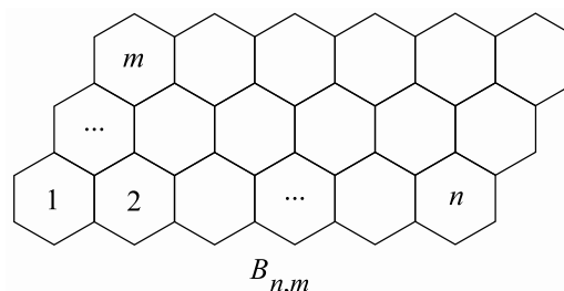
Figure 15. Benzenoid strip of length 6 and width 3.
