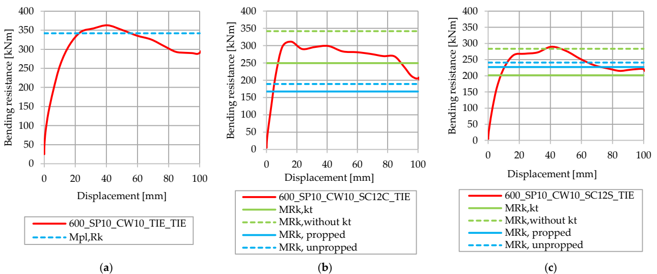
Figure 21. Comparison of analytical and numerical results of a steel beam height of 600 mm: (a) full shear connection; (b) shear connectors-in pairs; (c) shear connectors in a staggered arrangement.
