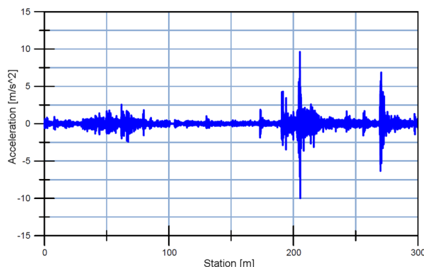
Fig. 6. Overhead wire shock time signal sample.
