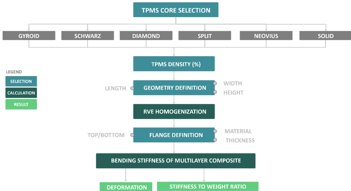
Figure 5.8 Design flowchart
