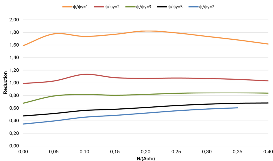
Figure 5. Influence of axial force on shear strength reduction.
