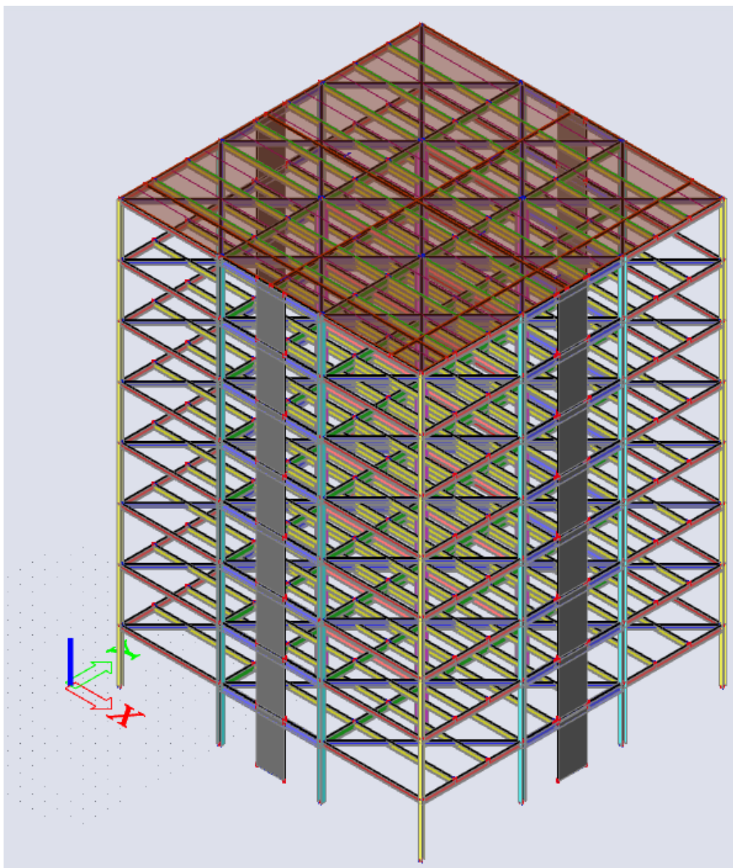
Slika 4.1 3D model
