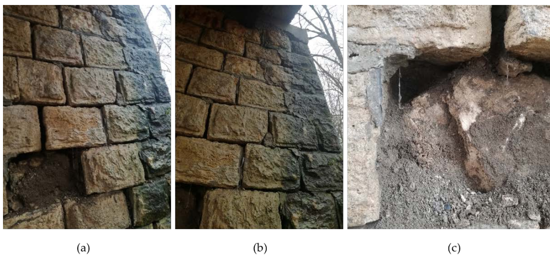
Figure 14. (a,b) Damage to the masonry walls of the abutment; (c) escarpment of infill material from the abutment.
