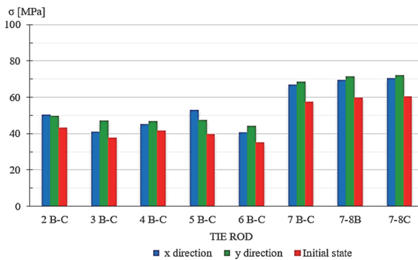
Figure 9. Comparison of stress level in iron tie-rods for the initial state and seismic actions in x and y-direction
