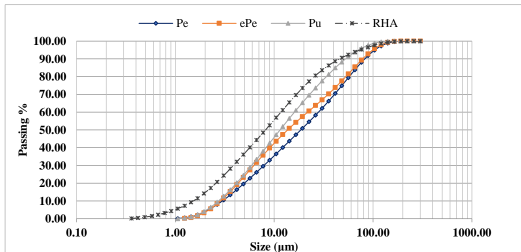
Figure 1: Particle size distribution of ground aggregates samples subjected to pozzolanicity test
