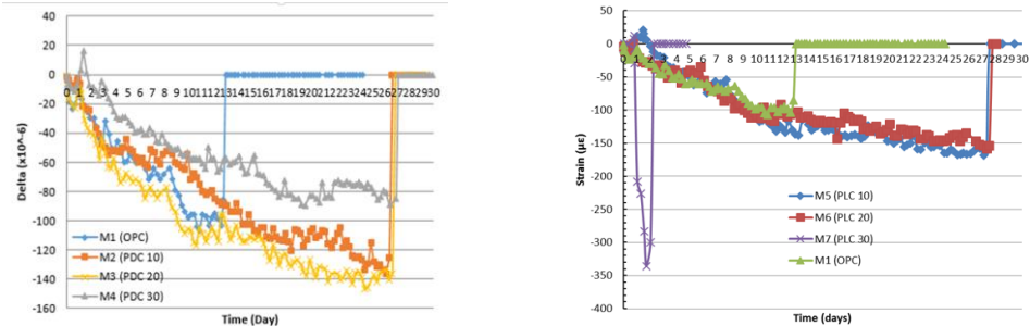
Figure 3: Relations between strain and time for ring samples for dolomite (left) and Limestone (right)
