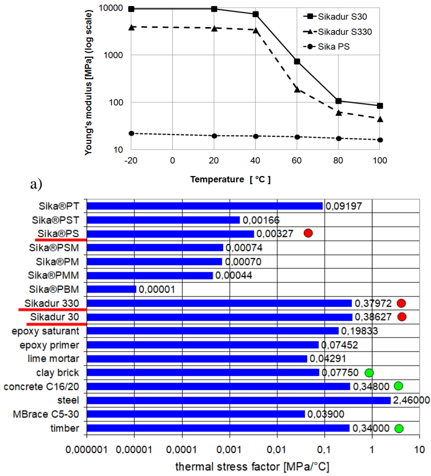
Figure 1: (a) Changes in stiffness of epoxy (S30, S330) and polyurethane (PS) adhesives with temperature and (b) values of thermal stress factors of structural materials
