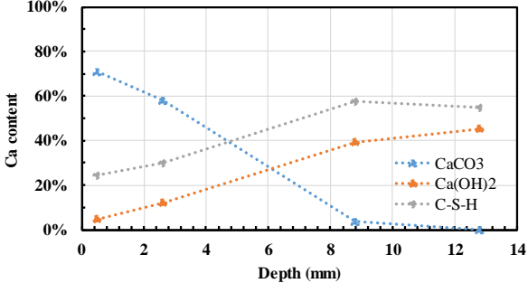
Figure 3 C/S = 3.0 38 days
