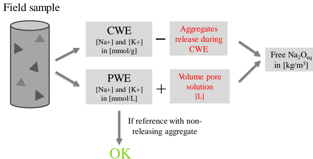
Figure 3 : Strategies for determination of alkali release from aggregates in concrete.
