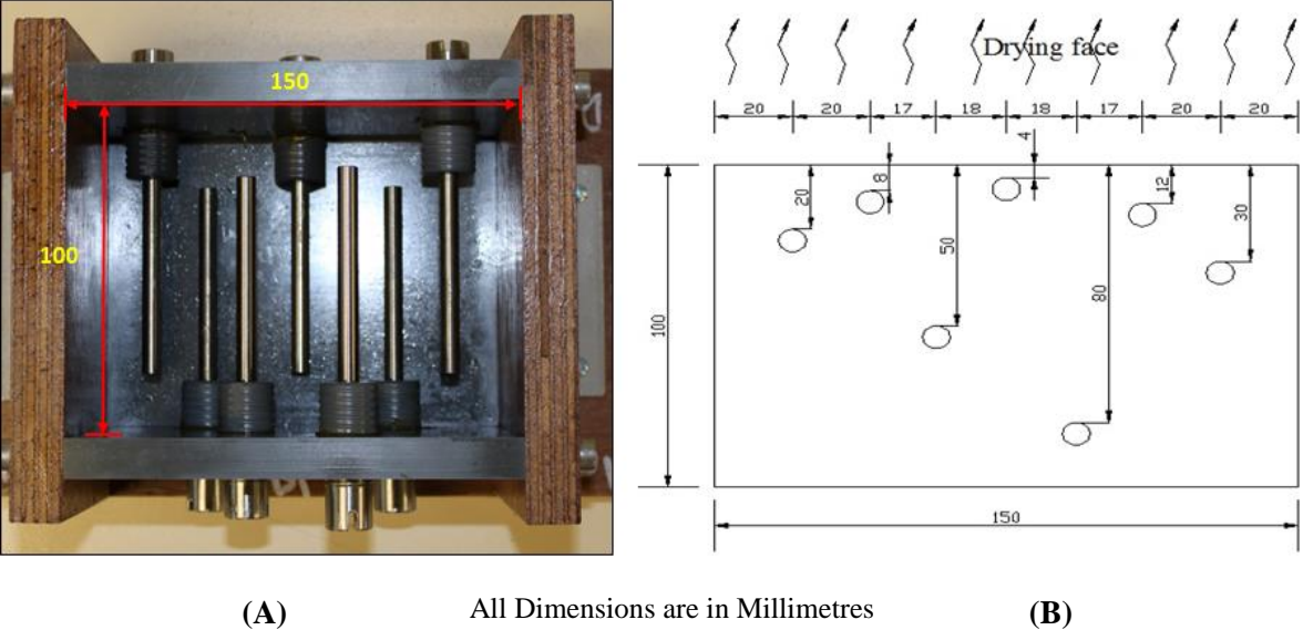
Figure 1: Arrangement of Cavities in Concrete Prism (A) Plan View of Mould used for Casting Concrete Specimens for Moisture Measurement, (B) Cross Section
