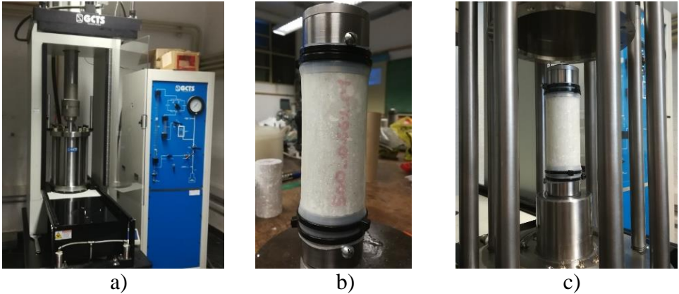
Figure 2: Equipment used to perform the multiaxial tests: a) general view of the GCTS equipment; b) detail of the sleeve to avoid direct contact with the oil; c) detailed view of a specimen prepared for triaxial testing.
