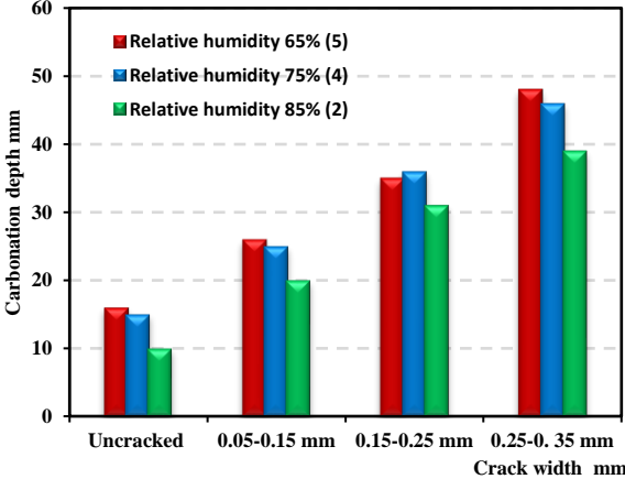
Figure 1-c: M 0.6 (w/c=0.6)
