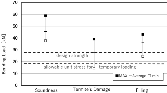
Figure 6: Result of bending test
