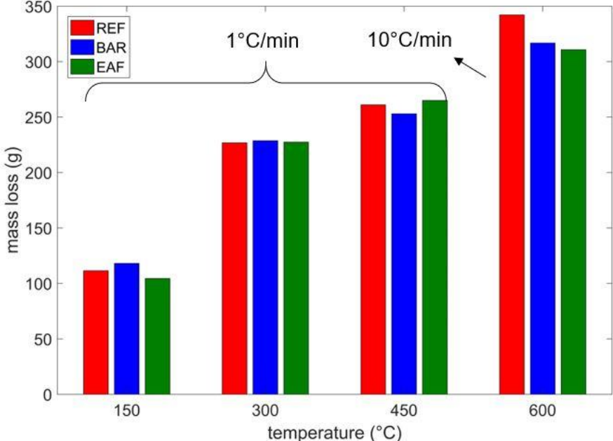
Figure 3: Mass loss of 100x200 mm concrete cylinders at slow heating rate (1°C/min – up to 450°C) and at moderate heating rate (10°C/min – 600°C).
