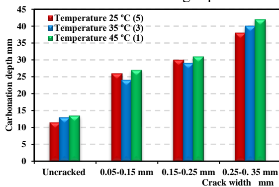
Figure 5-b:M 0.5
