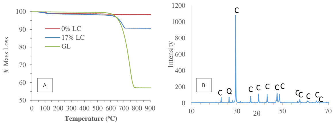
Figure 1: a) TG curves of 0% and 17% Limestone cement (LC) and Ground Limestone (GL) and b) XRD pattern of the ground limestone where C=calcite, CaCO 3 and Q=quartz
