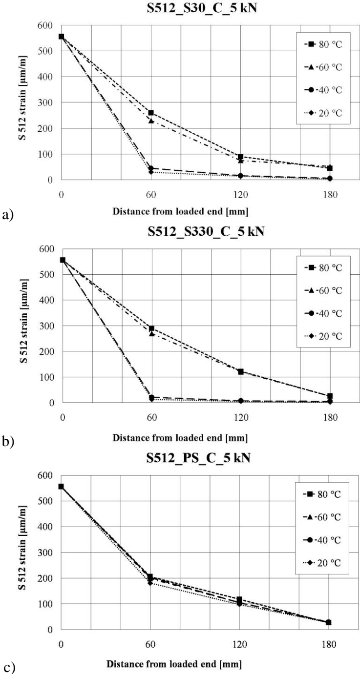
Figure 3: Strain distribution at S512 bonded to concrete substrate on epoxy S30 (a), S330 (b) and polyurethane Sika®PS (c), tested under load of 5 kN in temperatures: 20, 40, 60 and 80°C
