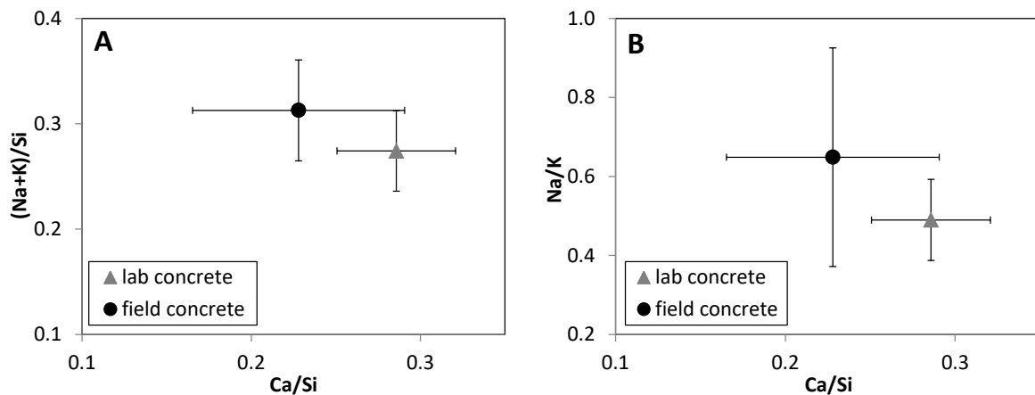
Figure 3: Molar (Na+K)/Si-ratio (A) and Na/K-ratio (B) as a function of the molar Ca/Si-ratio of the structured products in the field (unsheltered exposure case) and in the lab concrete.
