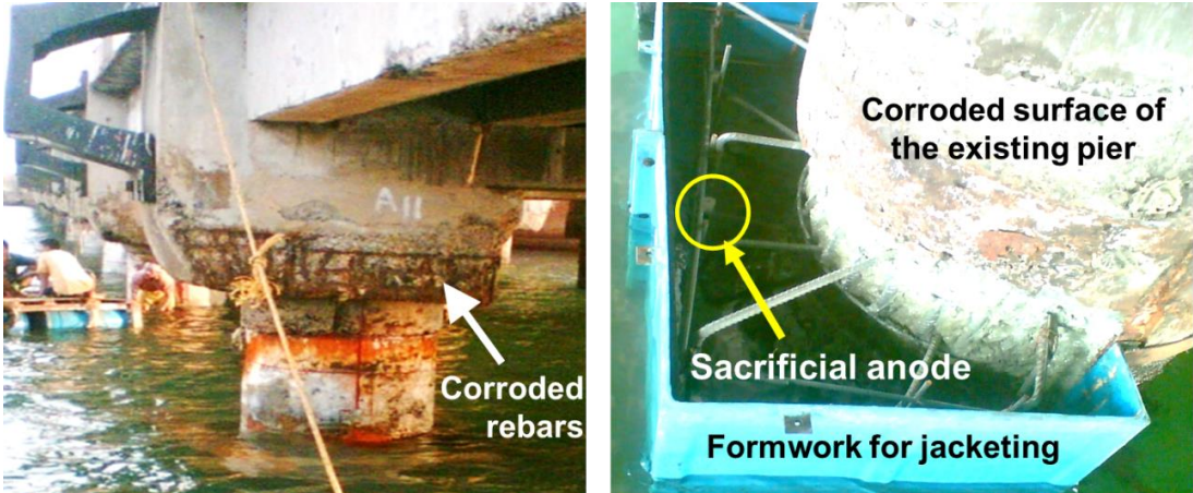
(a) Corroded rebars in a pier (circular cross-section) and pier cap (b) Setup for concrete jacketing with additional rebars and sacrificial anodes
