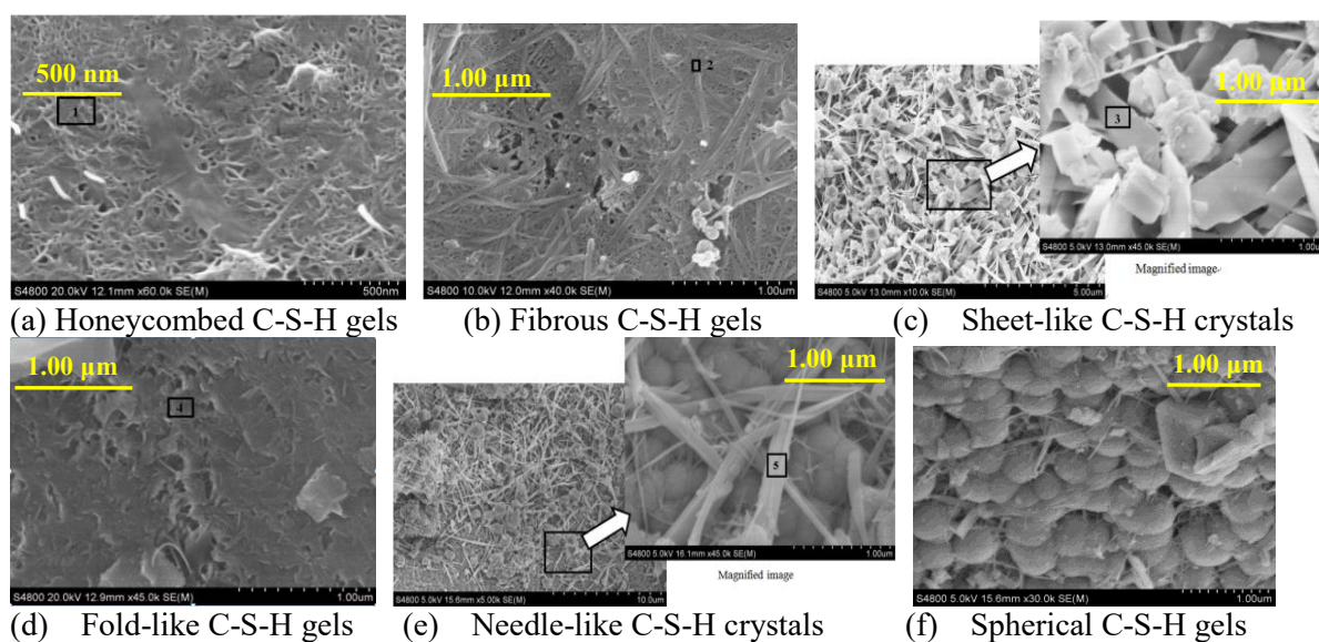
Fig. 4: Morphology of C-S-H in the samples subjected to various curing regimes
