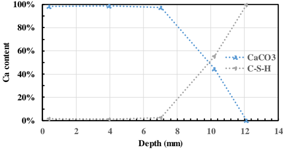
Figure 4 C/S = 1.4 28 days
