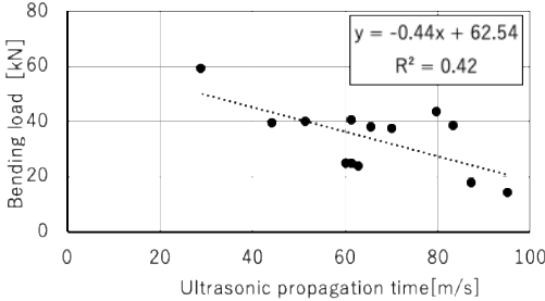
Figure 7: Bending load- ultrasonic propagation time
