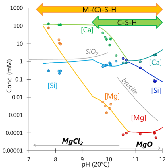
Figure 2: Effect of pH on the measured silicon, magnesium, and calcium concentrations at 20^{\circ}C . The solubility of M-S-H, C-S-H (solid lines), brucite and amorphous silica (grey lines) were calculated using thermodynamic modelling. Adapted from [10].
