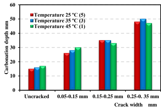
Figure 5-c: M 0.6
