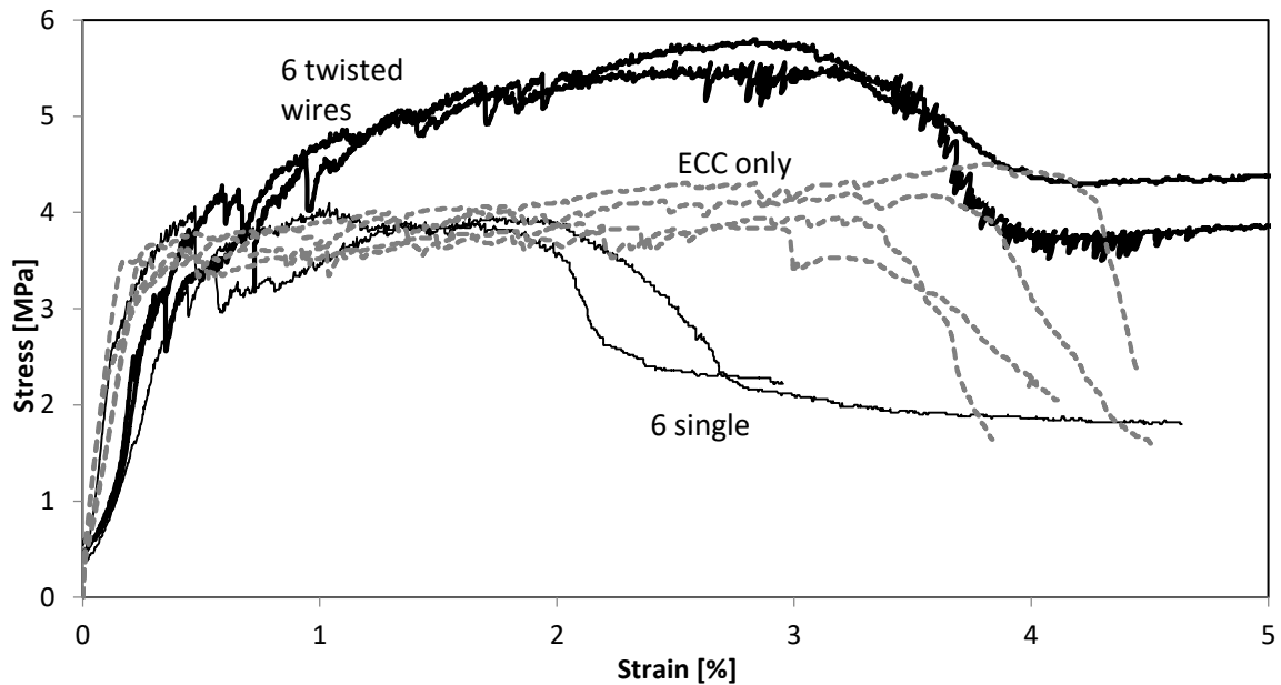
Figure 7: Tensile stress – strain responses of the ECC-Nitinol composites tested with single and twisted wires.
