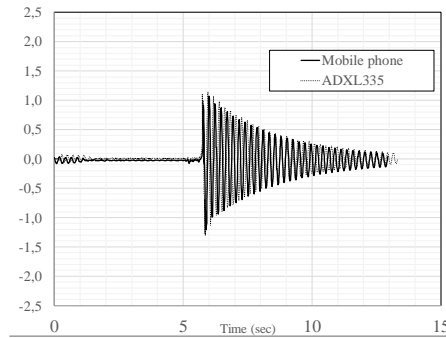
Fig. 3: Measured accelerations in the illustrative experiment on free vibrations
