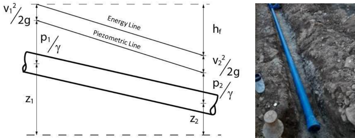
Fig. 3: Energy line – Piezometric line
