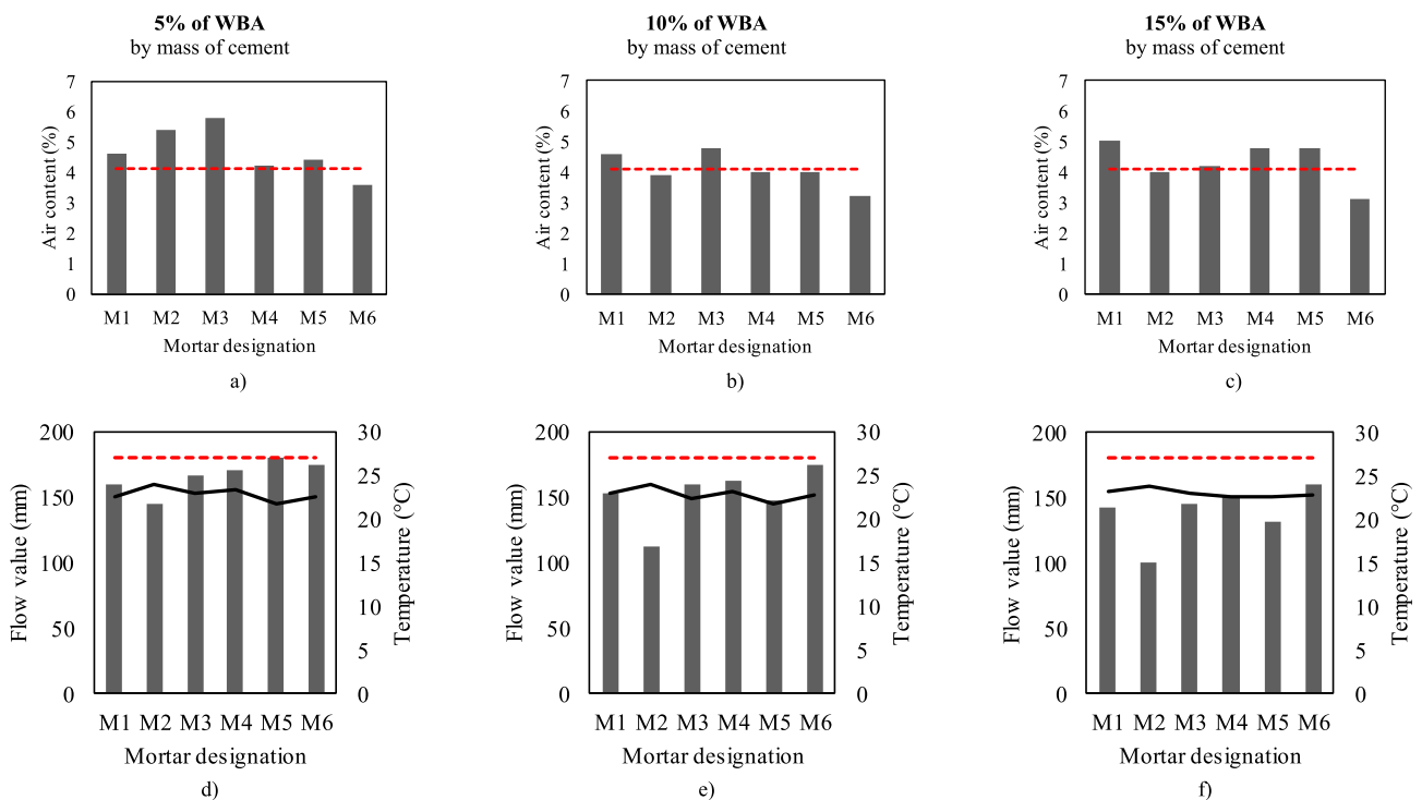
Fig. 2. Influence of WBA on properties of mortar based on WBAs type and content: a, b, c) Air content, d, e, f) Consistence (by flow table) and temperature (black line). ** red dashed lines in Figures a, b, c) represent air content of reference mix and in Figures d, e, f) flow value of reference mix.
