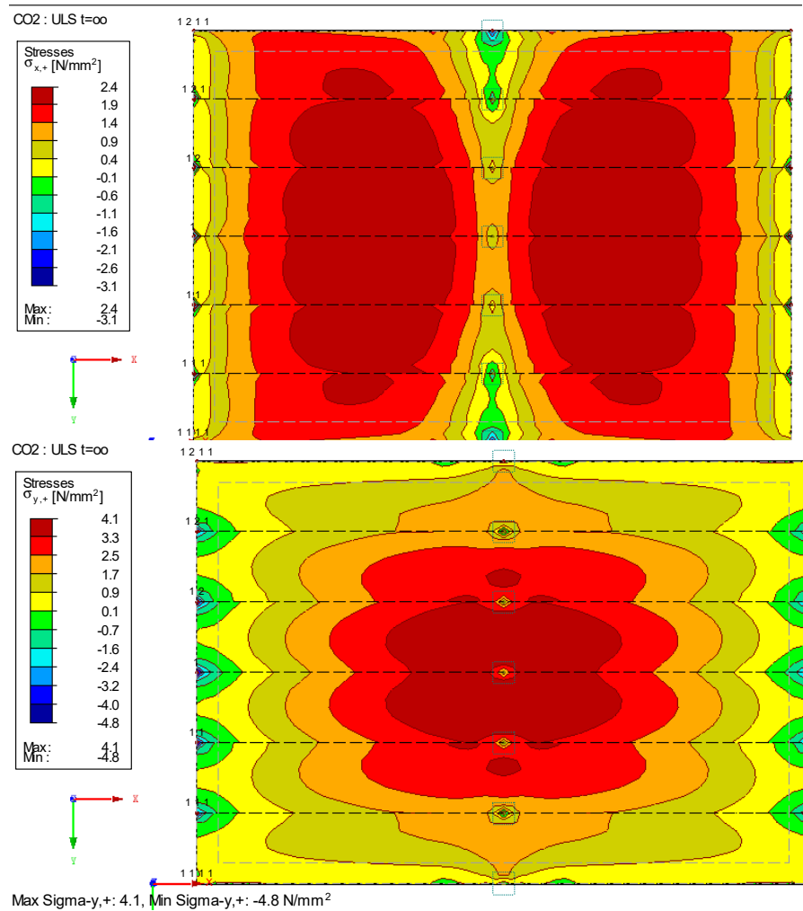
Figure 12. Concrete stresses.
