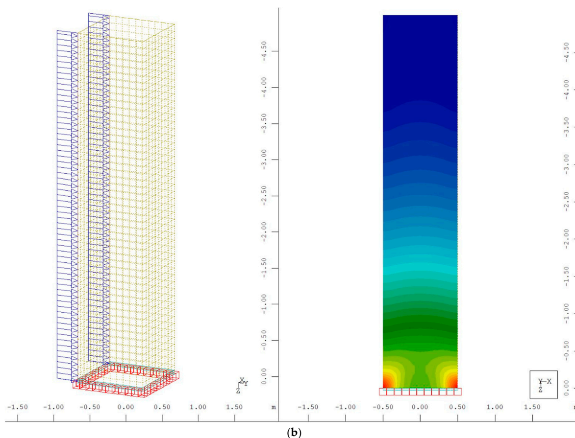
Figure 3. (a) Box section cantilever stress distribution for point load and (b) continuous load.
