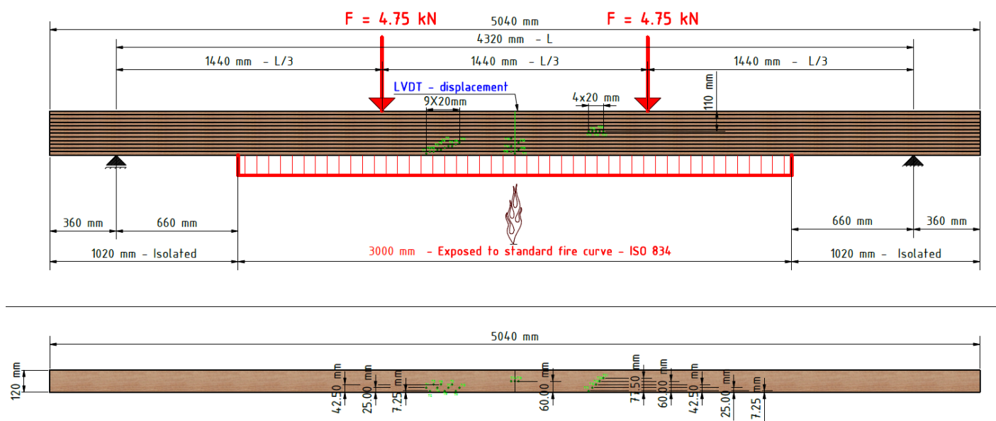
Figure 9. Fire test-experiment setup.
