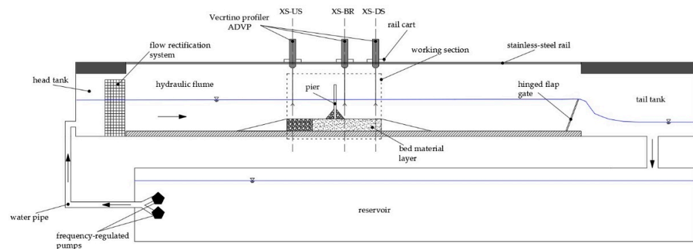
Figure 2. Scheme of the hydraulic flume setup.
