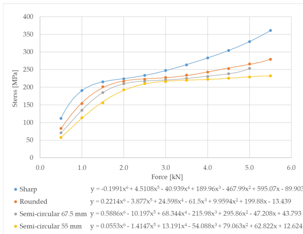
Figure 24. Von Mises stress–strain regression curves for \Delta\sigma_i .
