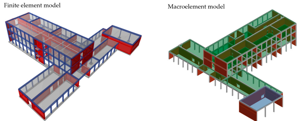
Figure 7. Numerical models of the building.
