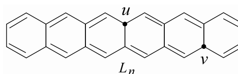
Figure 8. Unpaired electrons at vertices of degree 3.
