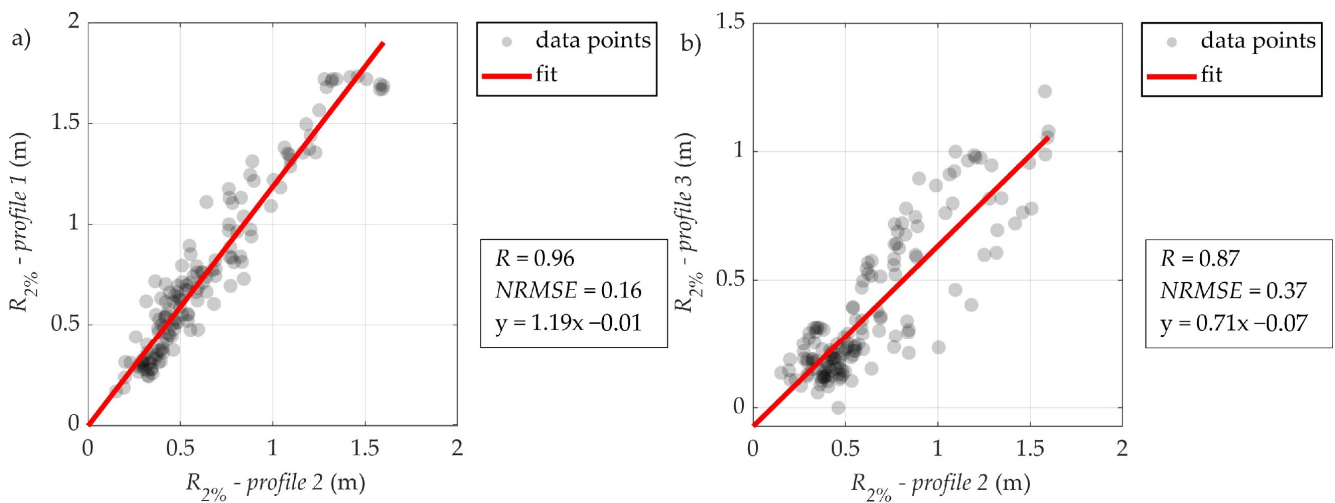
Figure 11. (a) Relationship between the wave runup, R_{2\%} , measured on the centerline profile (profile 2 in Figure 1d) and westward profile (profile 1 in Figure 1d); (b) Relationship between the wave runup, R_{2\%} , measured on the centerline profile (profile 2 in Figure 1d) and eastward profile (profile 3 in Figure 1d).
