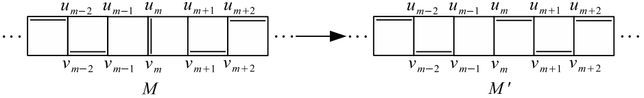
Figure 4: The case when u_{m-1} and u_{m+1} are both unsaturated.
