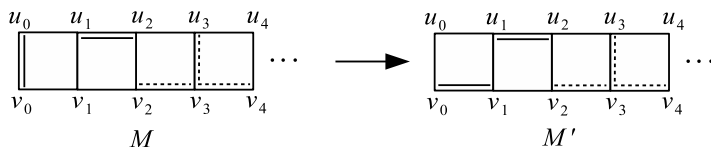
Figure 3: The case when m = 0 and only one of u_1, v_1 is saturated by M .
