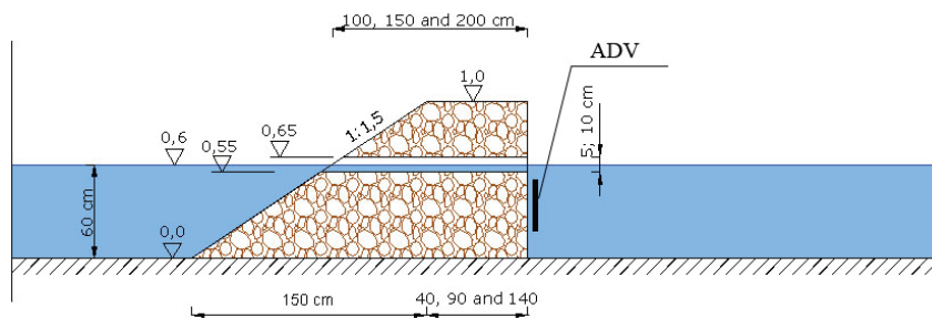
Figure 10 The longitudinal cross section and main dimensions of physical model built in wave flume
