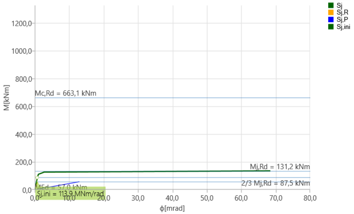
Stiffness diagram M_y - \phi
