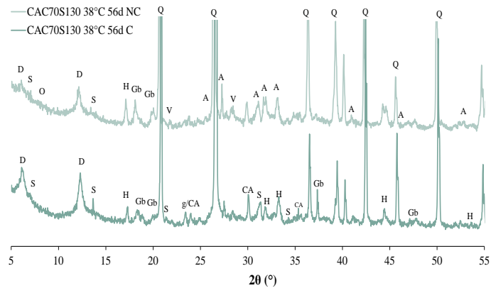
Figure 4.10 Diffractogram for non-carbonated and carbonated CAC70S130 38°C mix (CA=monocalcium aluminat, D=CAH10, Gb=AH3, G=Gehlenite, S=Strätlingite, H=C3AH6, O=C2AH8, Q=quartz, A=aragonite, C=calcite, V=vaterite)
